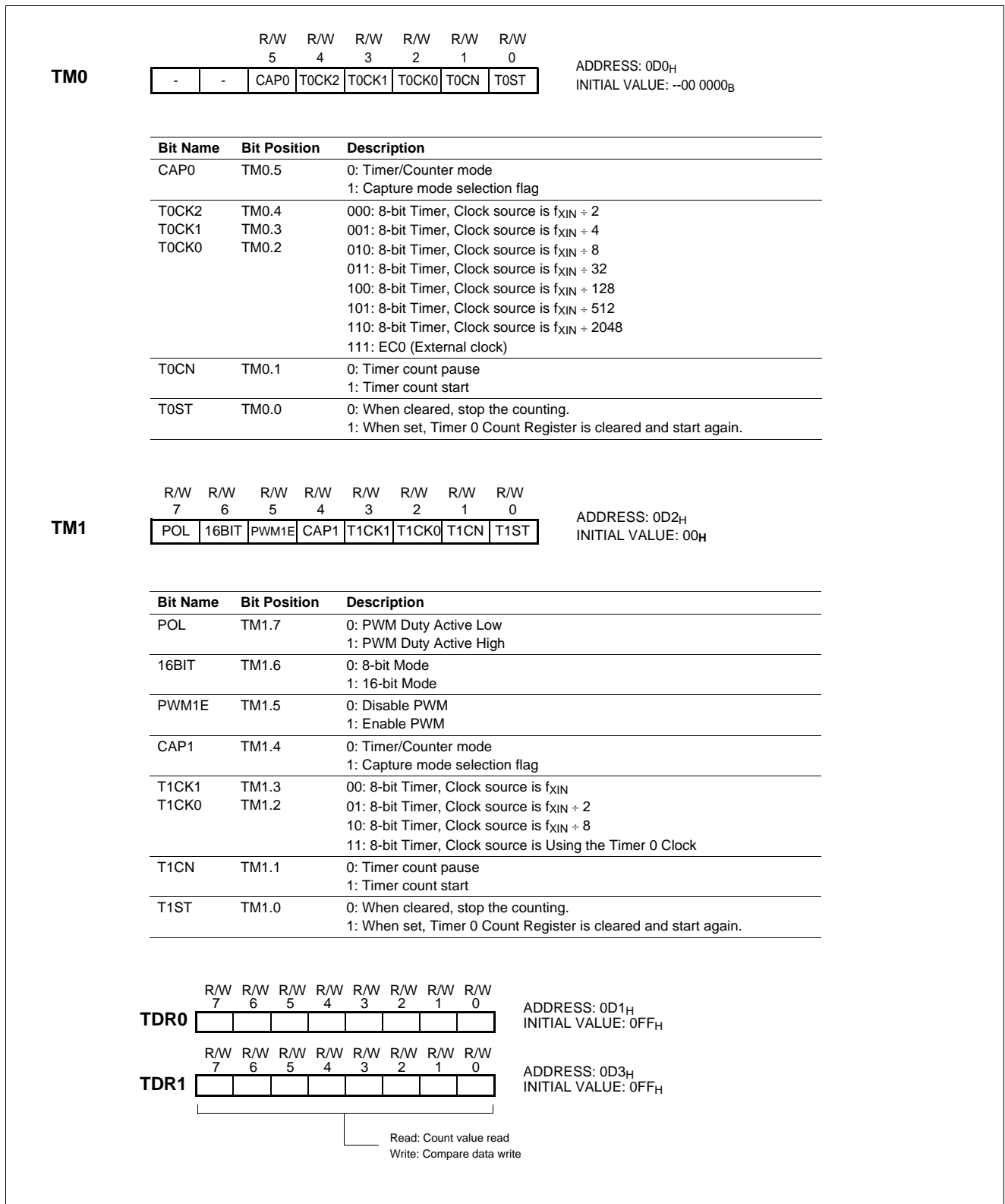
Figure 13-1 TM0, TM1 Registers
