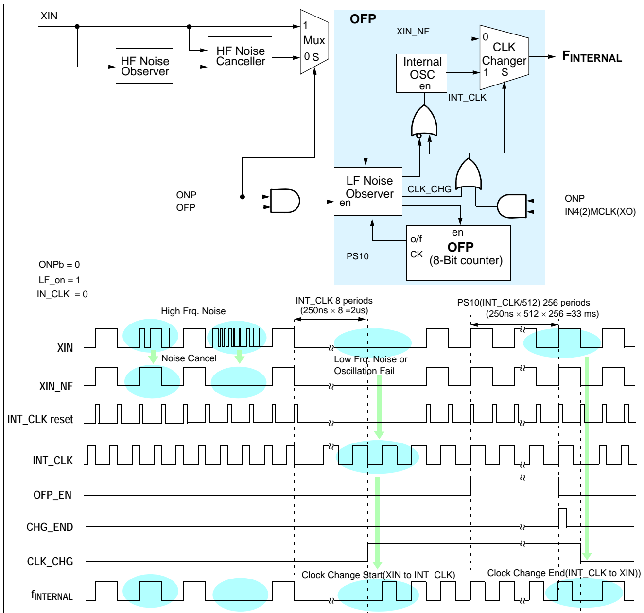
Figure 20-1 Block Diagram of ONP & OFF and Respective Wave Forms
