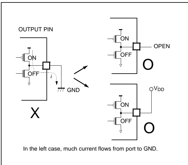
Figure 17-10 Application Example of Unused Output Port
